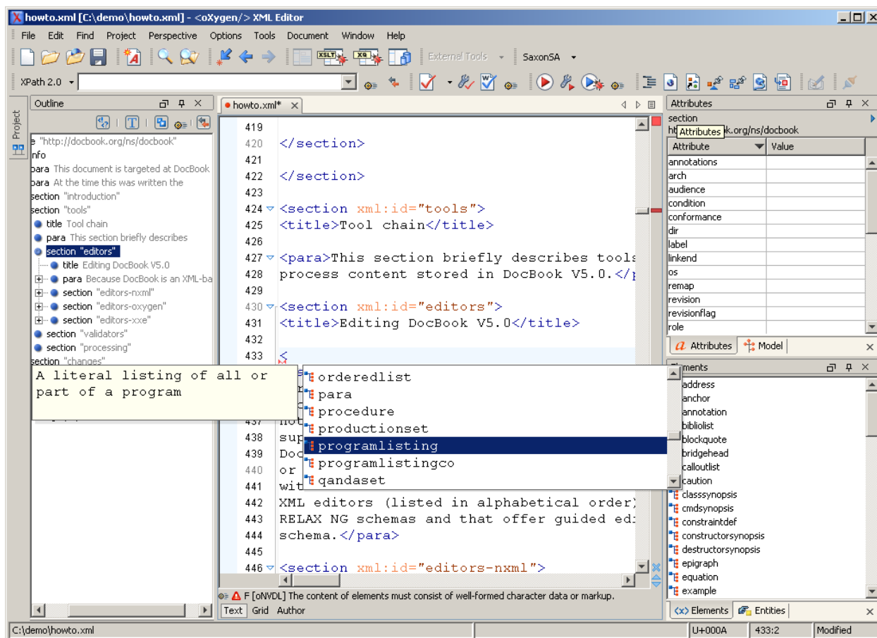
Figure 2. DocBook V5.0 document opened in oXygen
