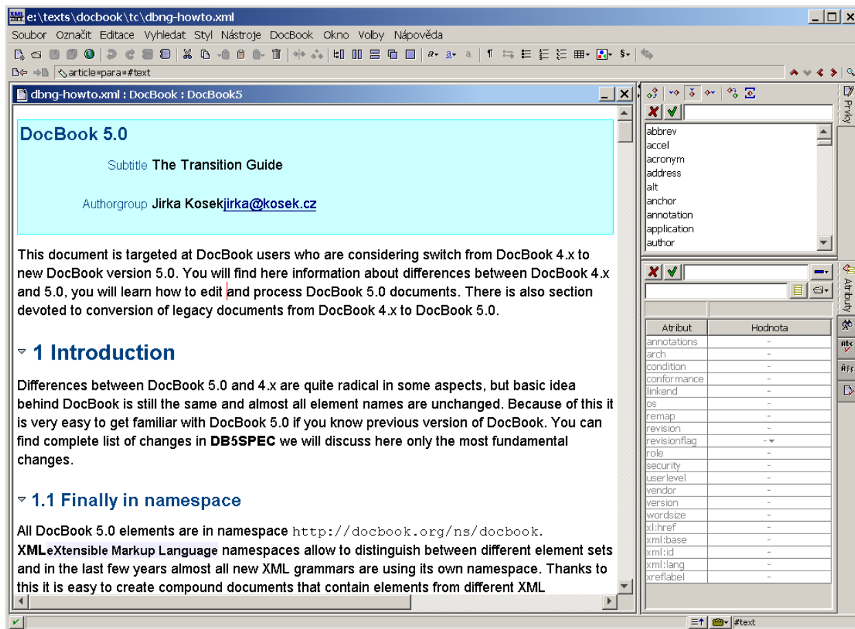
Figure 4. XML Mind XML Editor – feels almost like MS Word but real DocBook V5.0 markup is created
